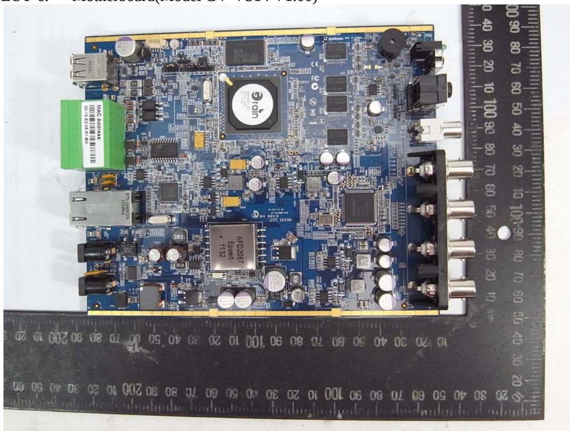
EUT-6. Motherboard(Model GV-VS14 V1.00)
